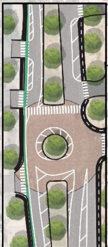
Typical Roundabout Striping
